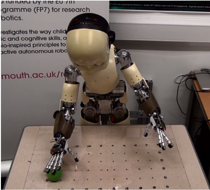
Fig. 3. Experimental setup
